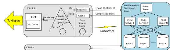
Figure 3: Client-server architecture.
