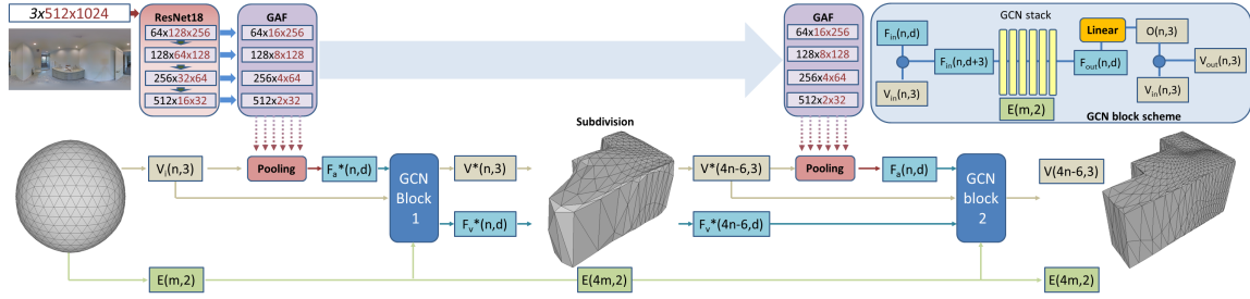
Figure 3. Our end-to-end deep learning technique maps an equirectangular image to a 3D mesh representing the bounding surface or the room. Two GCN blocks deform an input icosphere (Sec. 4.1) by offsetting its vertices (see Sec. 4.2). The first block starts from a first pooling of the GAF features F^*(n, d) to return a low-res estimation of the mesh M^*(V^*, E_i) . This low-res representation M^* is then refined to poll refined GAF features F^*(4n - 6, d) , which drive the second GCN block. The output of the second block is the final refined mesh model M(V(4n - 6, 3), E(4m, 2)) .
