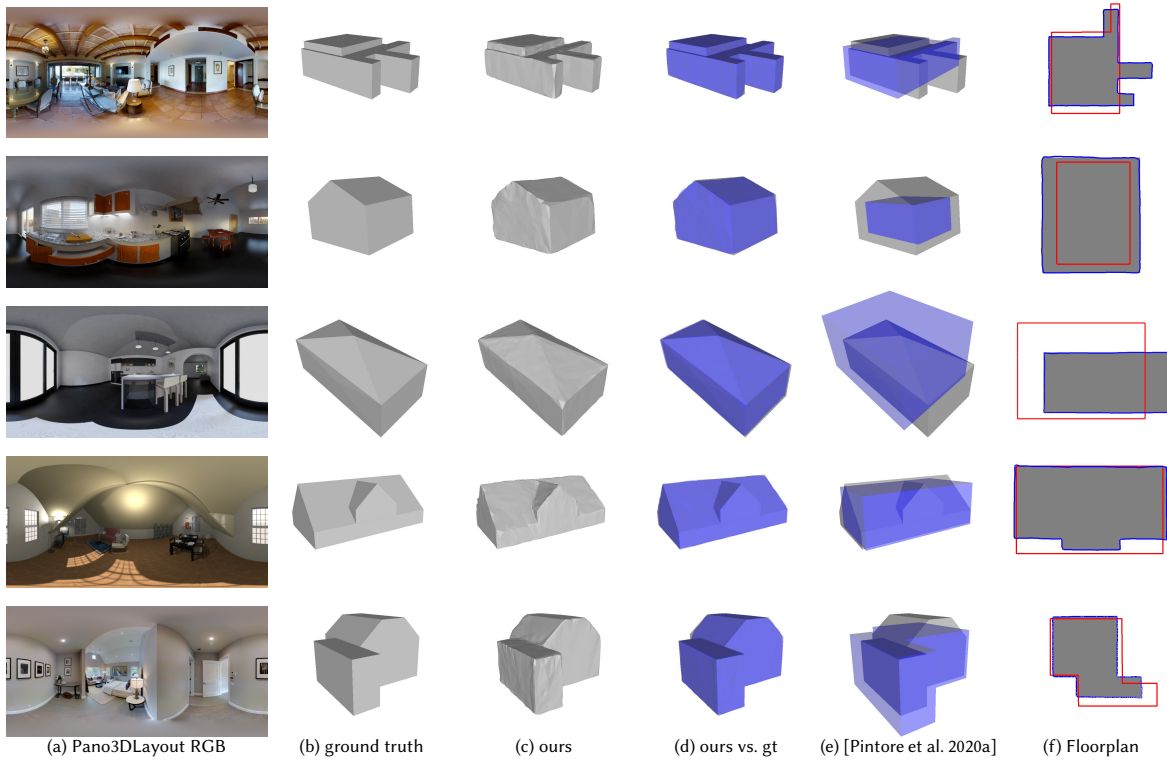
Figure 7. Qualitative comparison on non-MWM scenes ( Pano3DLayout ). We show the input image, the ground truth model, our prediction, our prediction in overlay with ground truth, competitor prediction in overlay with ground truth and the 2D floorplan comparison (grey ground truth, blue ours, red competitor). Our approach has consistent performance for a variety of model kinds, in particular for complex structures, such as domes and sloping roofs.
