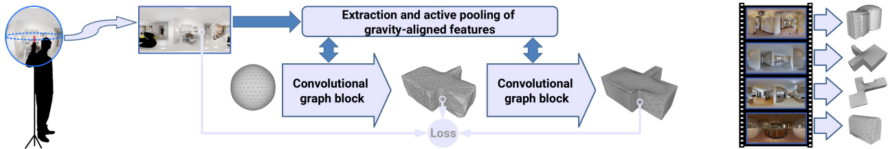
Figure 1. From a single cluttered panoramic image, our end-to-end deep network recovers, at interactive rates, a watertight 3D mesh of the underlying architectural structure. The graph convolutional network, trained using indoor-specific losses, exploits multi-scale gravity-aligned features and active pooling to deform a tessellated sphere to the correct geometry. Reconstructed models may include curved walls, sloped or stepped ceilings, domes, and concave shapes.
