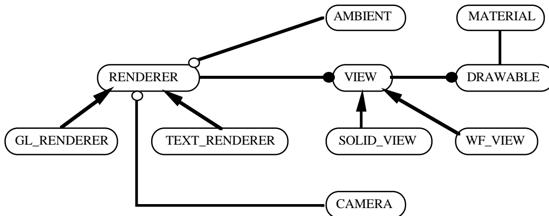
Fig 3: Basic rendering classes
