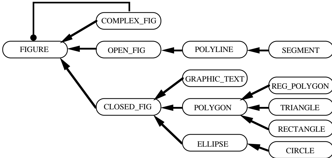
Fig 1: Two dimensional figures
