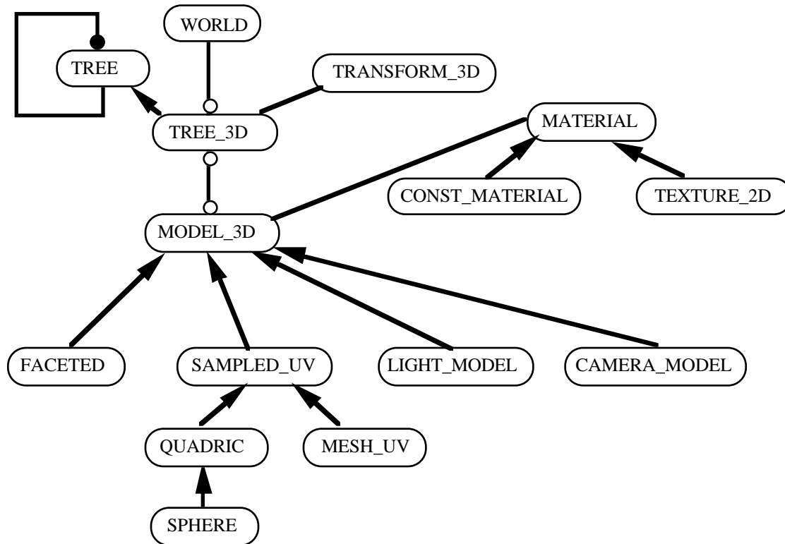
Fig. 2: Basic modeling classes
