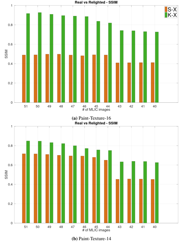
Figure 3: We use SSIM metric to compare the performance of the single pixel strategy S-X with our k-neighbor based solution K-X. The graphs show the worst SSIM value in the relighted MLIC obtained from SV-BRDFs computed after removing from one to twelve images from the original 52 image MLIC. The more images are removed, the worse is the relighting quality. However, our solution can always provide better performances than the state-of-the-art single pixel approach.
