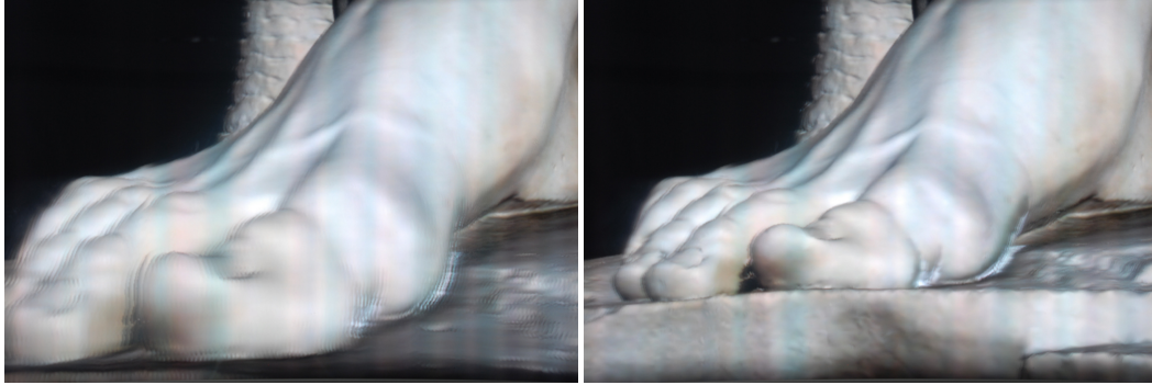
Figure 5: Depth compression. Left: rendering quality for object portions too far from the screen surface is insufficient because of limited spatial accuracy and precision in calibration. Right: non-linear depth compression reduces artifacts while minimizing modification of shape in the neighborhood of the screen surface.
